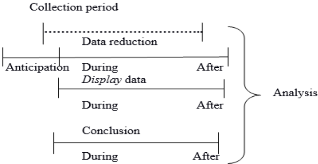
Figure 1. Research flowchart
